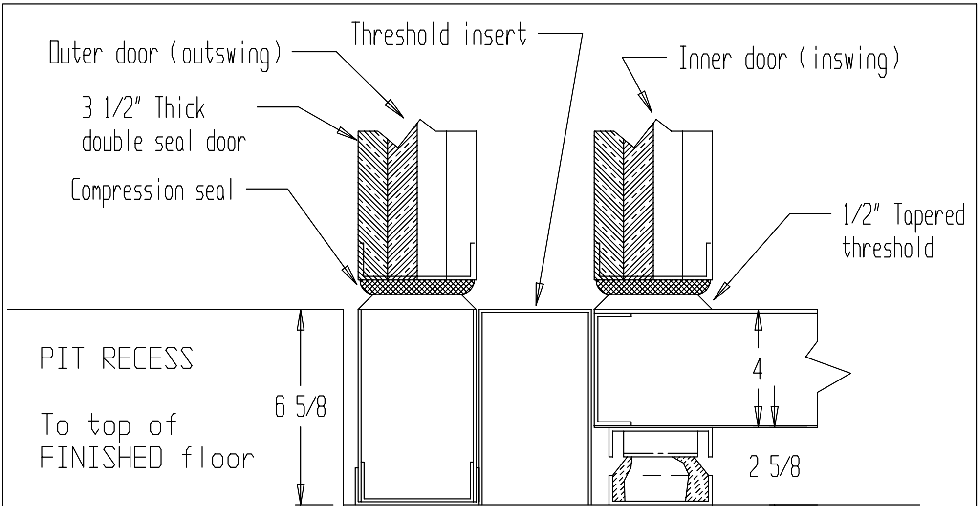
Double Wall Exam Booth Pit / Threshold Detail 4" Floor with 2 5/8" Isolation Rails
